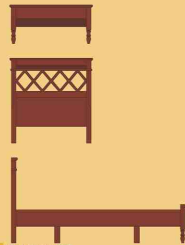
1. Pat simplu 900 Simple bed 900 1010 x 2130 x 1030/463
